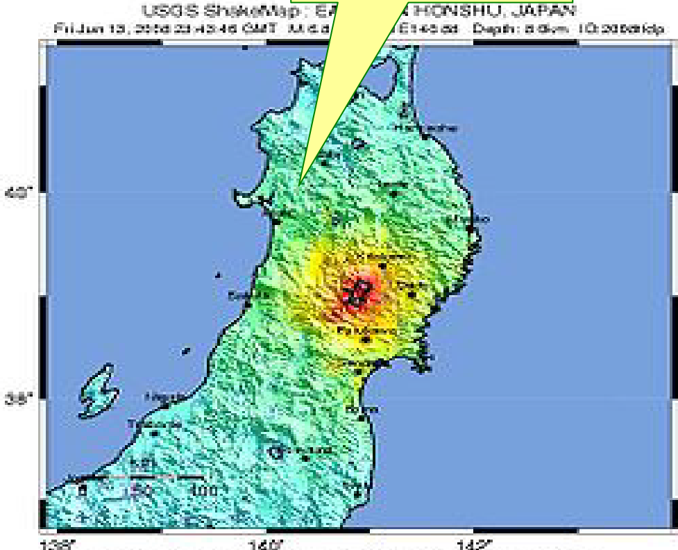
USGS ShakeMap: Earthquake of 2008 JUN 14 08:43:46 GMT, Honshu, Japan. Epicenter: 38.2°N, 141.2°E, Depth: 8.0km, 10:2008Jp
